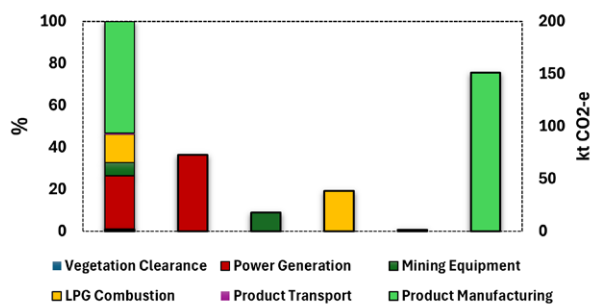
GHG Emissions from a Typical Metalliferous Mine for One Year Period
